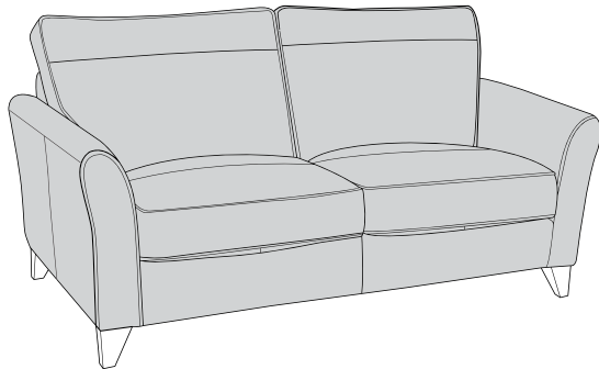
2 Seater Sofa: 2S H: 102 W: 157 D: 97
